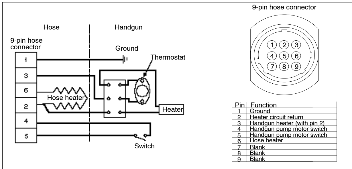
Figure 20 Wiring Diagram
