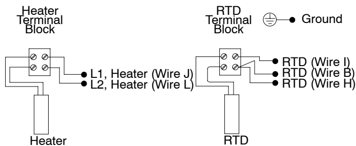
Figure 6 Wiring Diagram
