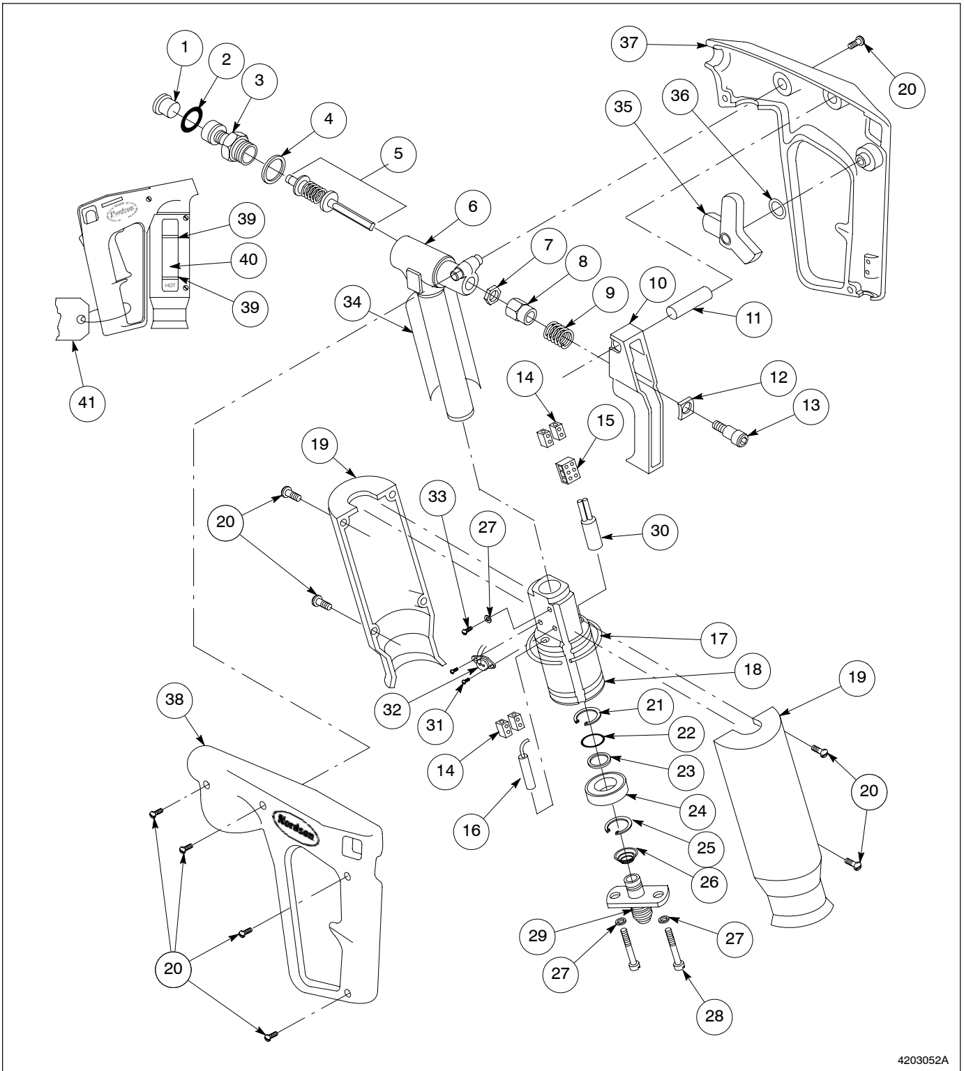
Figure 51 AD-31 Models A, T, and TL Handgun Parts
