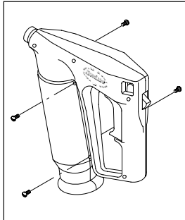
Figure 2 Remove Pivot Sleeve Shells (typical gun shown)
