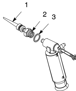
Figure 43 Nozzle Assembly (typical nozzle shown)
